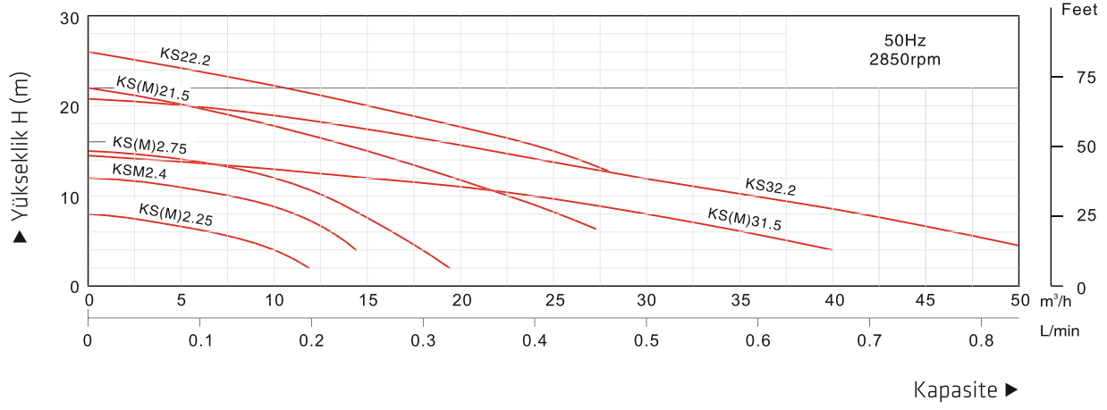
Performans Eğrisi - Performance Curves
