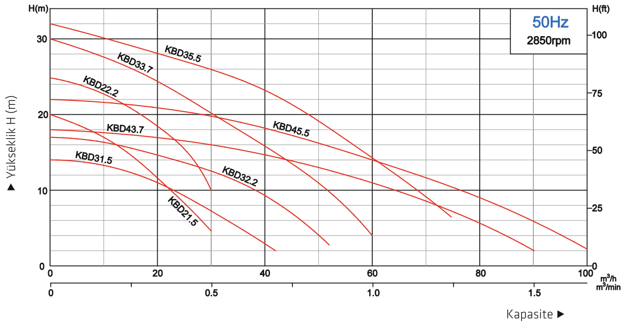
KBD Serisi Performans Eğrisi - KBD Series Performance Curves
